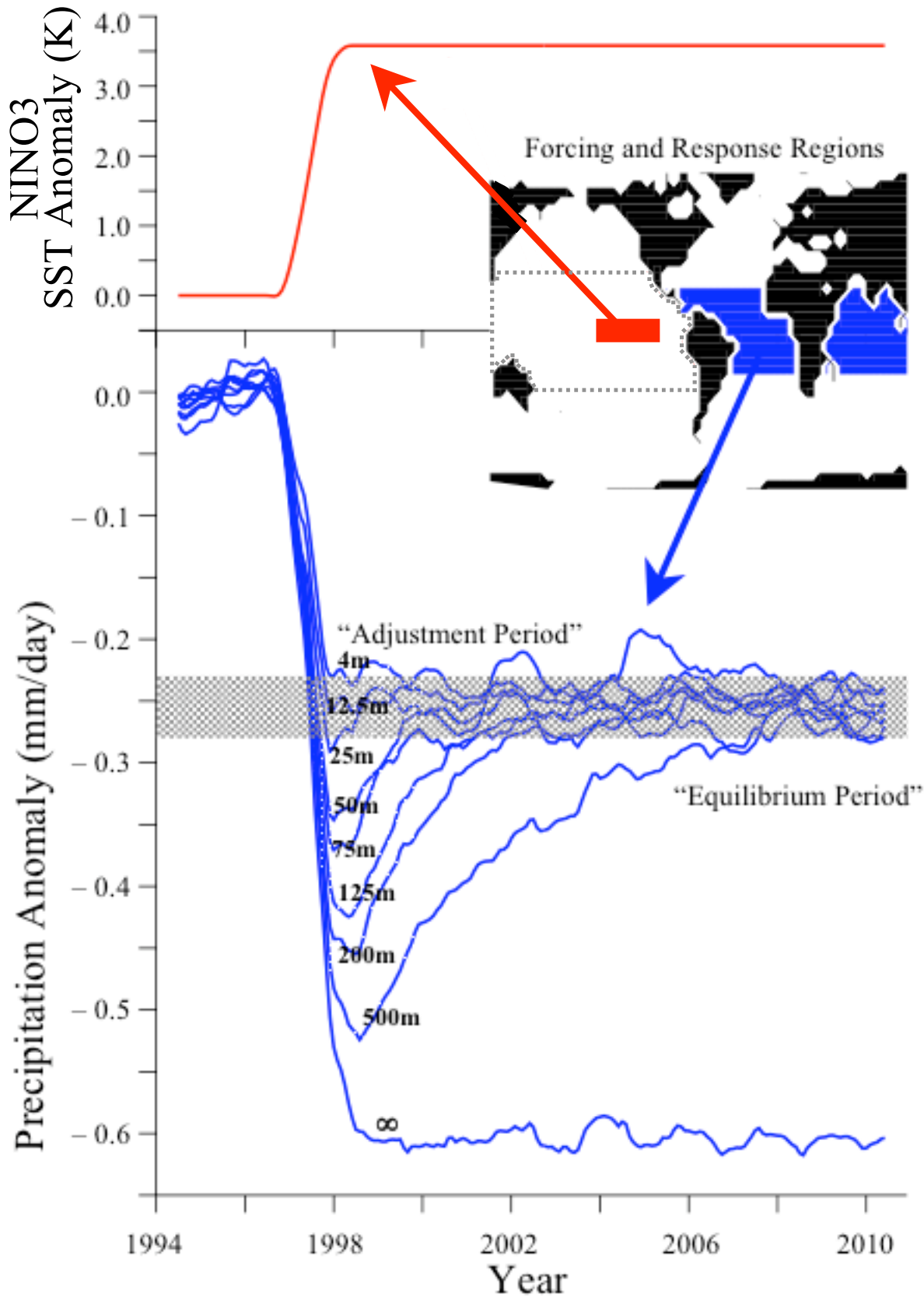
Remote Ocean Precipitation Response
